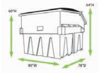
6 YARD FL FLAT TOP
