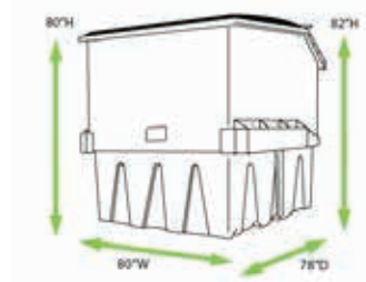
8 YARD FL FLAT TOP
