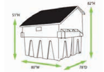
8 YARD FL SLANT TOP
